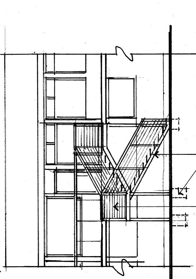
SECTION D-D. SCALE 1:100
